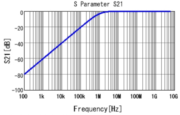
■ GRM033B31H152KA12 S21 DCOV, 20degC
