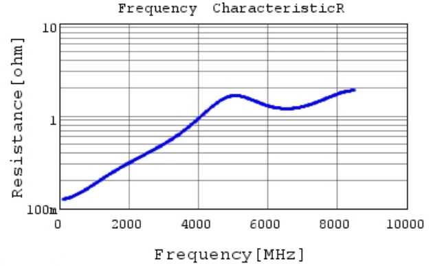
GRM0335C2A620JA01 R DCOV, 25degC
