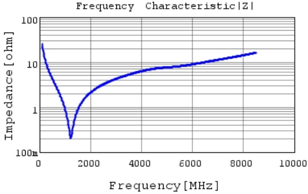
GRM0335C2A620JA01 |Z| DCOV, 25degC
