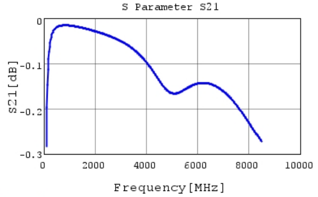
GRM0335C2A620JA01 S21 DCOV, 25degC
