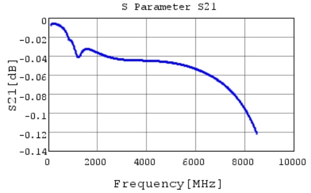
GRM0332C1E681JA01 S21 DCOV, 20degC
