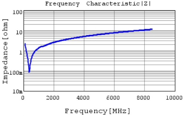
GRM0332C1E681JA01 |Z| DCOV, 20degC
