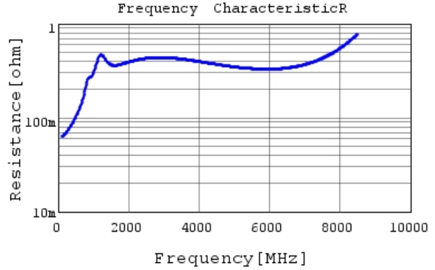
GRM0332C1E681JA01 R DCOV, 20degC
