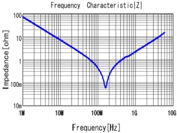
■ GRM1551X1A222JA01 |Z| DCOV, 20degC
