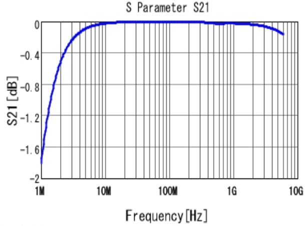
■ GRM1551X1A222JA01 S21 DCOV, 20degC
