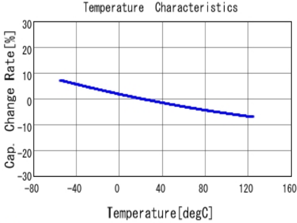
■ GRM1551X1A222JA01 C-Temp. capchange, DCOV, AC1Vrms
