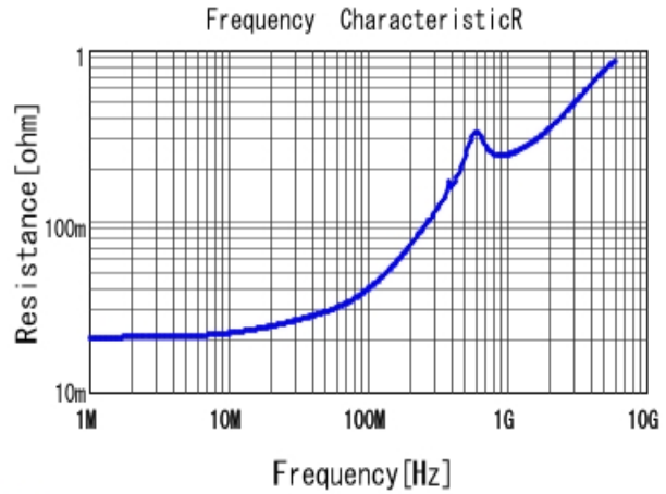
■ GRM1551X1A222JA01 R DCOV, 20degC
