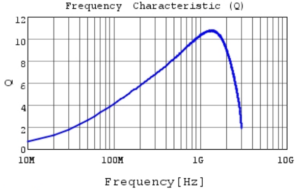
LQP02TN22NH02 Q
