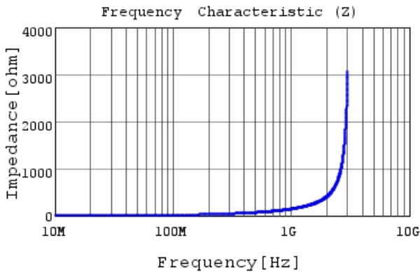
LQP02TN22NH02 |Z|
