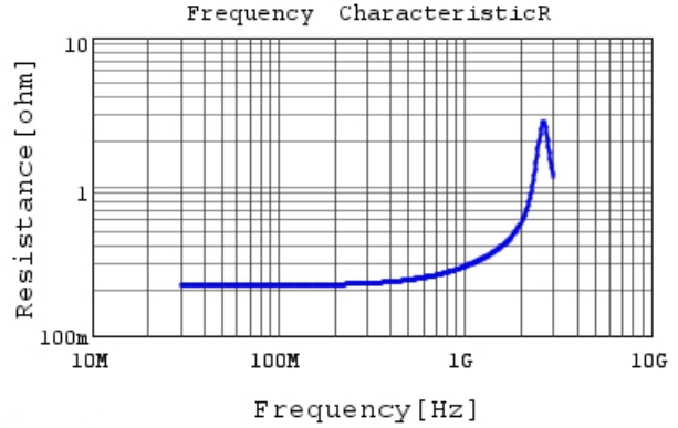
RDE5C2A330J0P1H03B R DC0V, 25degC
