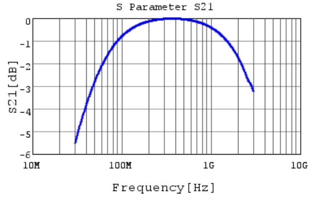
RDE5C2A330J0P1H03B S21 DCOV, 25degC
