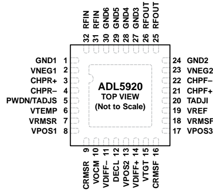
Figure 2. Pin Configuration
