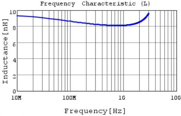
LQP02HQ8N2J02 L
