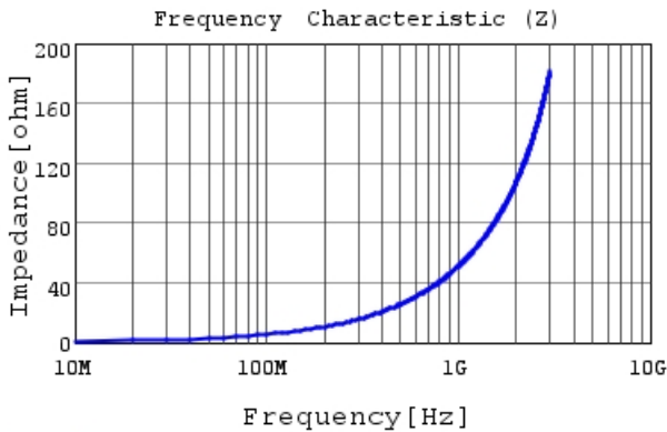
LQP02HQ8N2J02 |Z|
