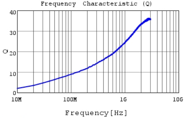
LQP02HQ8N2J02 Q
