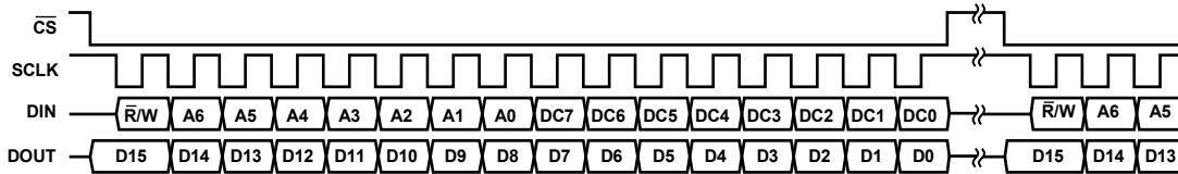
Figure 44. SPI Multibyte Read Command Example
