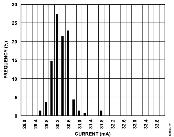
Figure 23. Operating Mode Current Distribution at 3.3 V Supply
