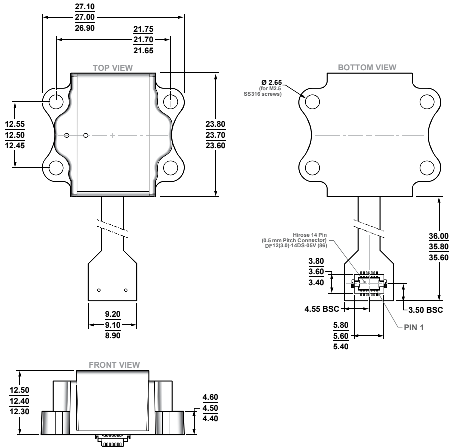
Figure 54. 14-Lead Module with Integrated Flex Connector [MODULE] (ML-14-7) Dimensions shown in millimeters
