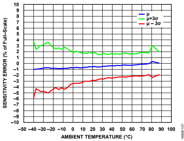
Figure 20. Sensitivity Error vs. Temperature
