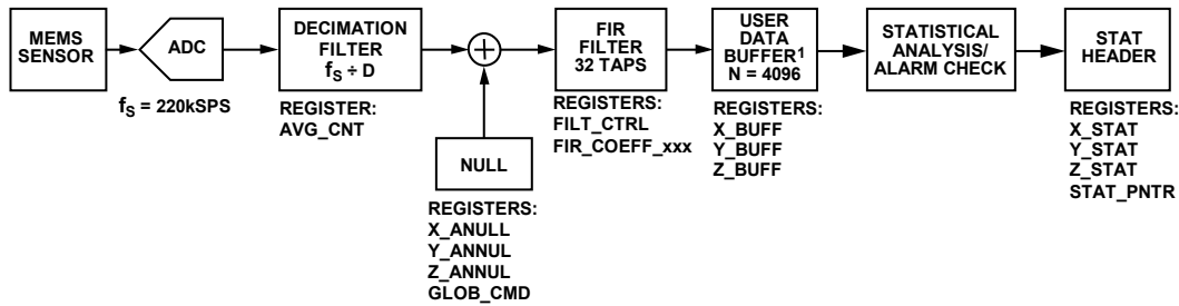
Figure 49. MTC Mode Datapath Processing
