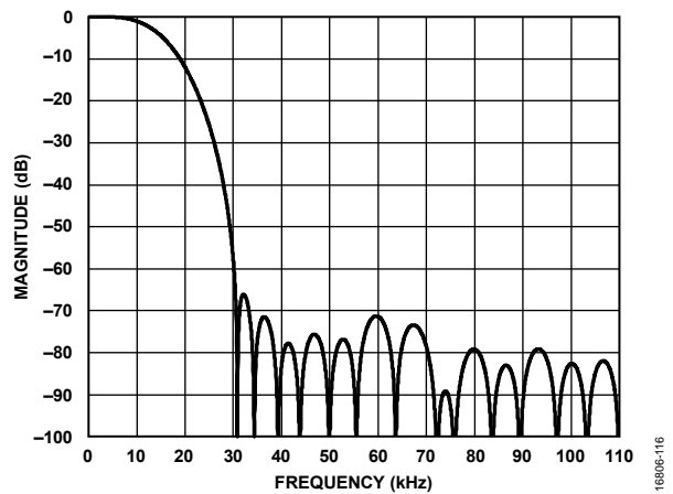
Figure 29. Digital Filter Frequency Response of the 5 kHz Low-Pass Filter
