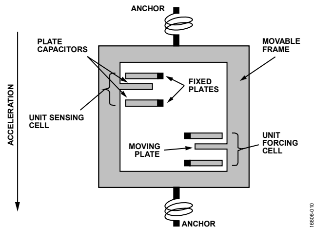
Figure 35. MEMS Sensor Diagram
