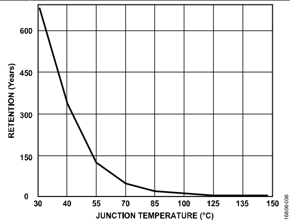
Figure 53. Flash/EE Memory Data Retention
