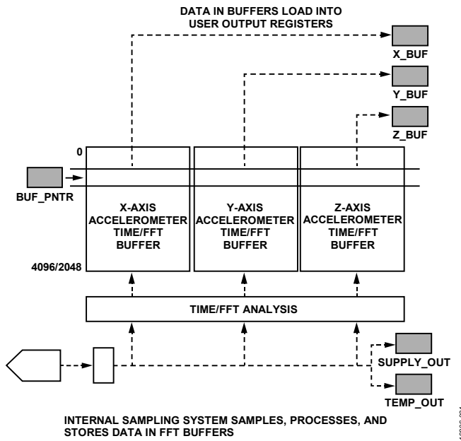
Figure 39. Data Buffer Structure and Operation
