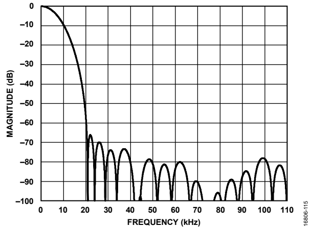
Figure 28. Digital Filter Frequency Response of the 1 kHz Low-Pass Filter
