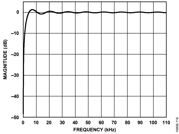
Figure 31. Digital Filter Frequency Response of the 1 kHz High-Pass Filter
