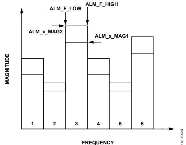
Figure 51. Spectral Alarm Band Registers
