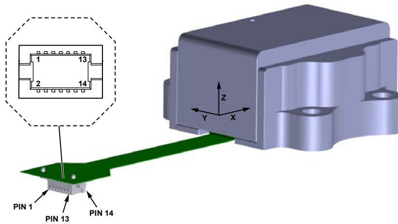
Figure 6. Pin Configuration
