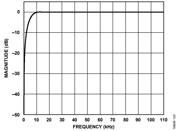
Figure 33. Digital Filter Frequency Response of the 10 kHz High-Pass Filter
