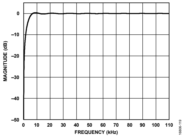
Figure 32. Digital Filter Frequency Response of the 5 kHz High-Pass Filter
