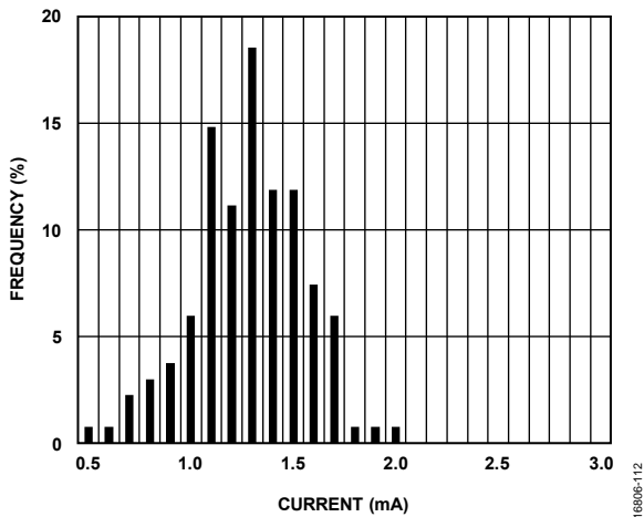
Figure 26. Sleep Mode Current Distribution at 3.3 V Supply
