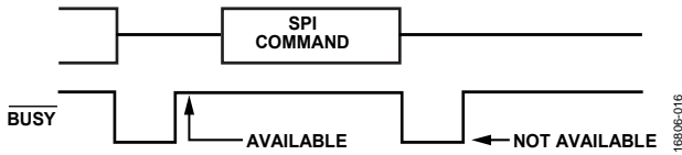
Figure 46. Busy Signal ( \overline{\text{BUSY}} ) Orientation after SPI command
