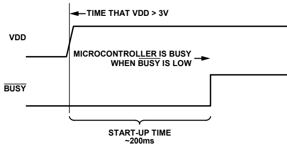
Figure 47. \overline{\text{BUSY}} Response During Startup
