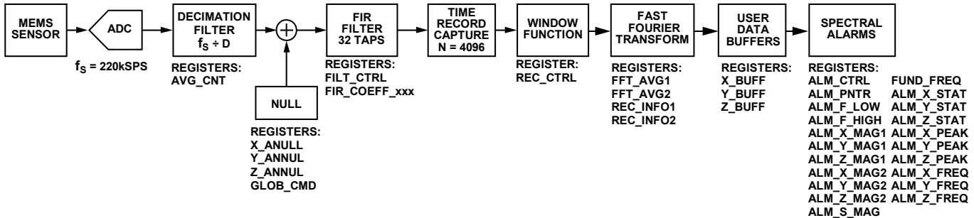
Figure 50. AFFT Mode and MFFT Mode Datapath Processing
