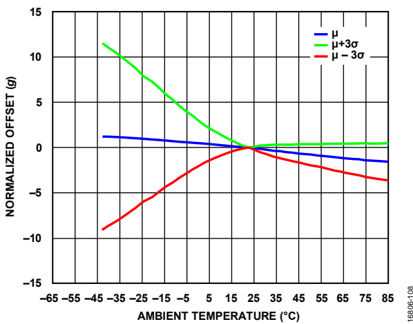
Figure 21. Offset vs. Temperature
