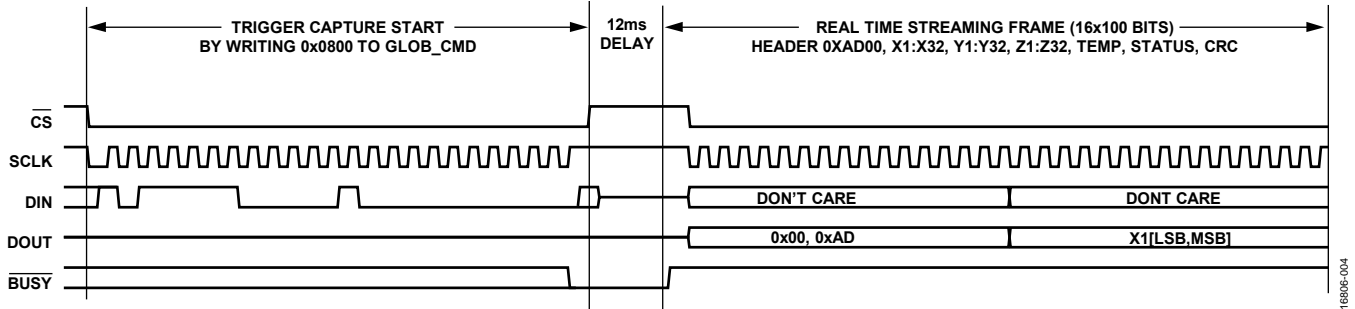
Figure 4. RTS Mode Timing Diagram (Assumes REC_CTRL, Bits[1:0] = 0b11)
