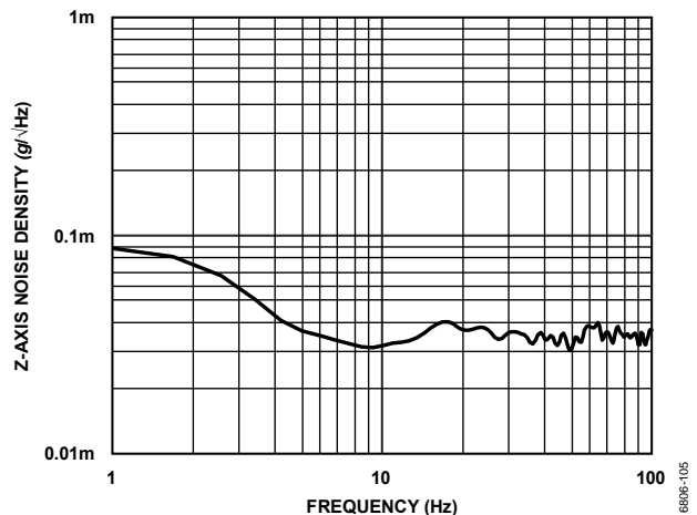
Figure 18. Z-Axis Noise Density, Low Frequency, RTS Mode
