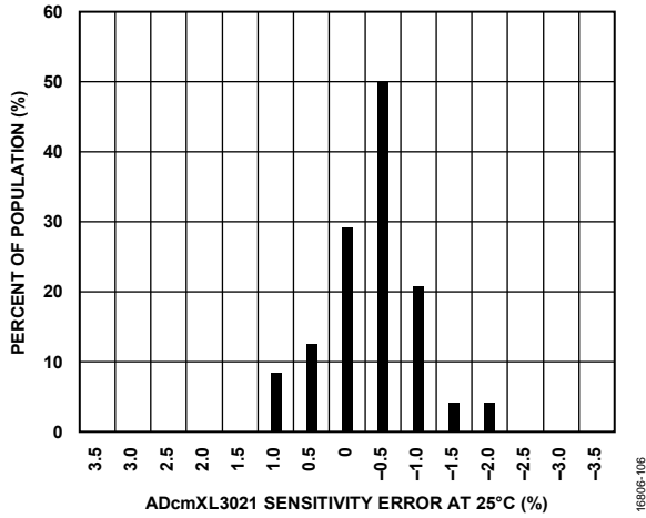
Figure 19. Sensitivity Distribution Histogram at 25°C
