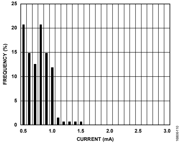
Figure 25. Sleep Mode Current Distribution at 3.0 V Supply
