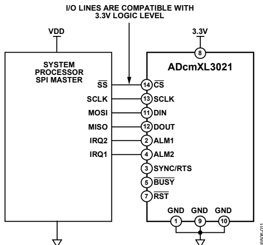
Figure 41. Electrical Hookup Diagram
