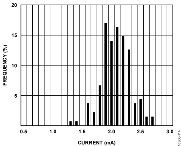
Figure 27. Sleep Mode Current Distribution at 3.6 V Supply
