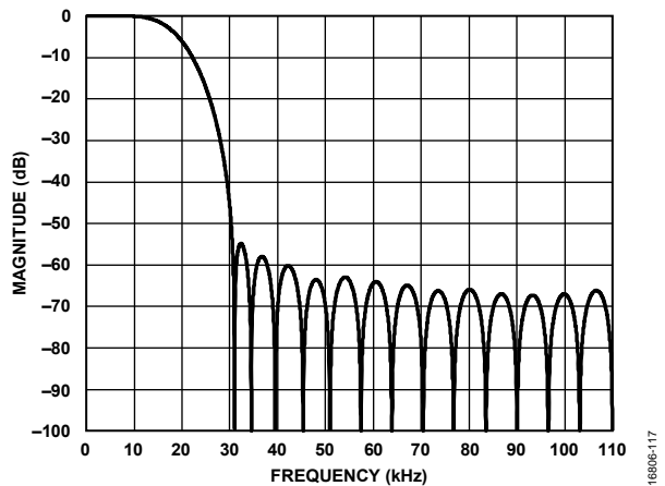
Figure 30. Digital Filter Frequency Response of the 10 kHz Low-Pass Filter
