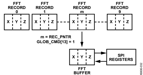
Figure 40. FFT Record Access
