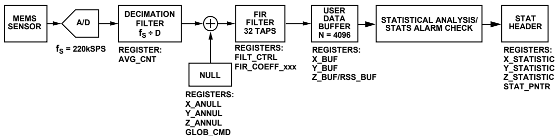
Figure 37. MTC Signal Flow Diagram
