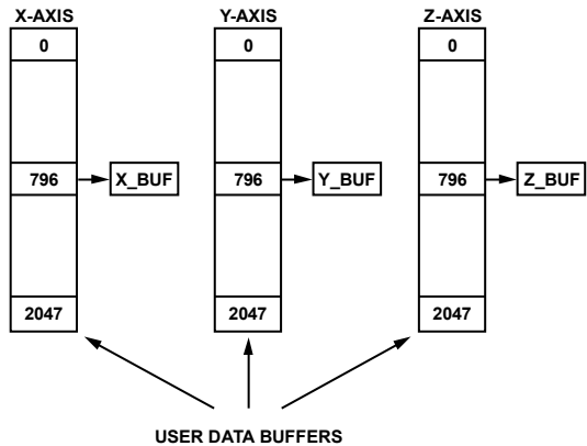
Figure 52. Register Activity, BUF_PNTR = 0x031C (MFFT Mode or AFFT Mode)
