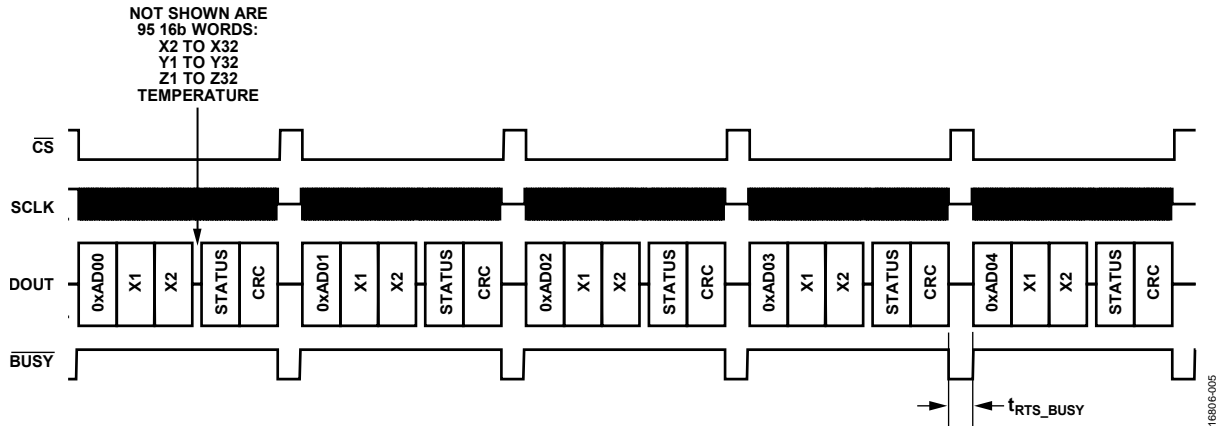
Figure 5. Burst Read Function Sequence Diagram, First Five Segments
