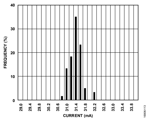
Figure 24. Operating Mode Current Distribution at 3.6 V Supply
