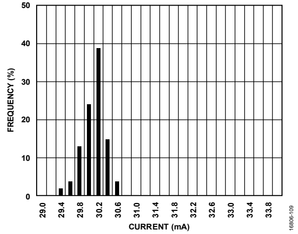
Figure 22. Operating Mode Current Distribution at 3.0 V Supply
