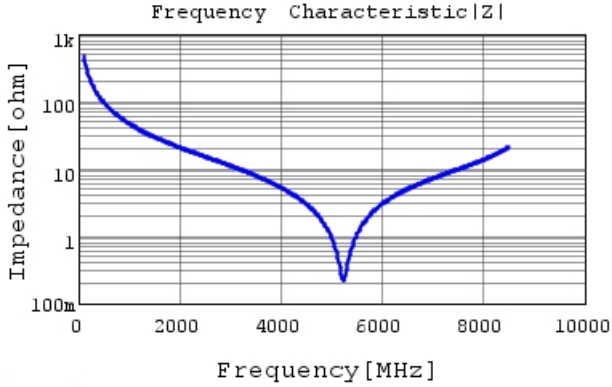
GQM1555C2D3R3CB01 |Z| DC0V, 25degC
