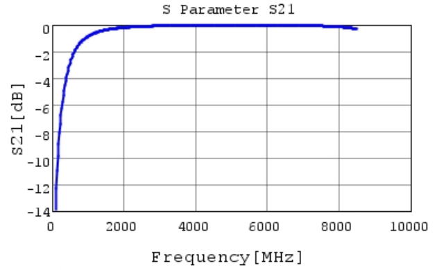
GQM1555C2D3R3CB01 S21 DCOV, 25degC
