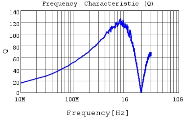
LQW2UAS47NF0C Q
