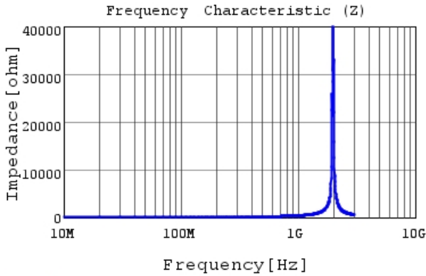
LQW2UAS47NF0C |Z|
