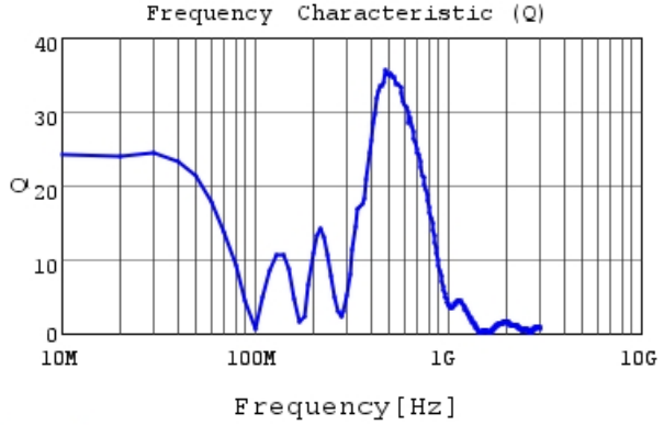
LQW2UAS4R7J0C Q
