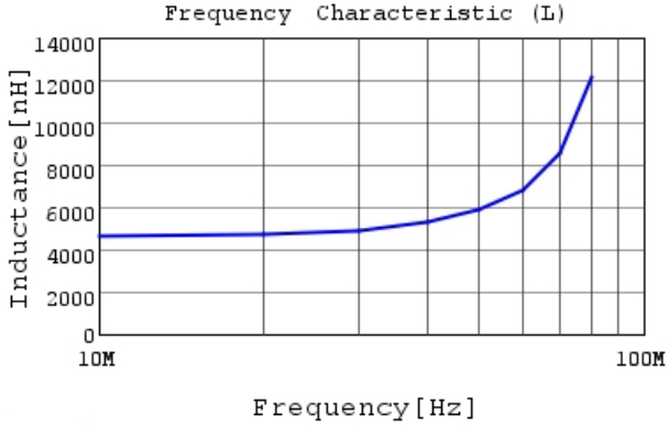
LQW2UAS4R7J0C L
