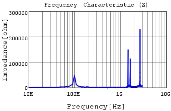
LQW2UAS4R7J0C |Z|
