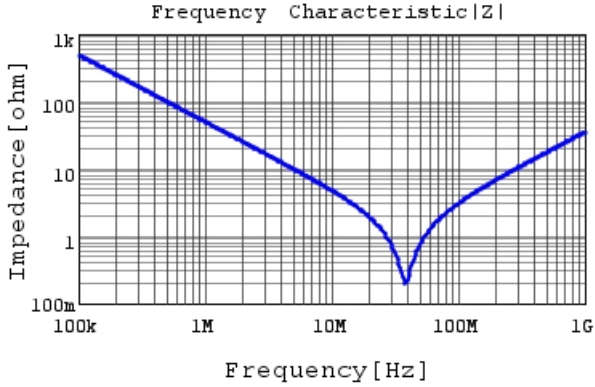
RDER72A332K0P1H03B |Z| DCOV, 25degC
