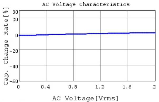
RDER72A332K0P1H03B C-AC Voltage capchange, I
