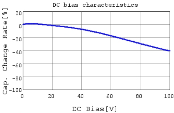
RDER72A332K0P1H03B C-DC bias capchange, 25.0
