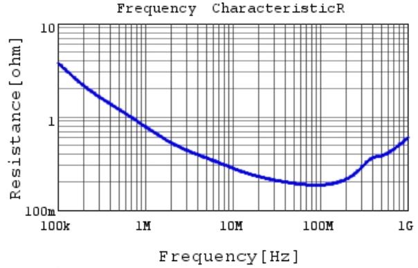
RDER72A332K0P1H03B R DCOV, 25degC
