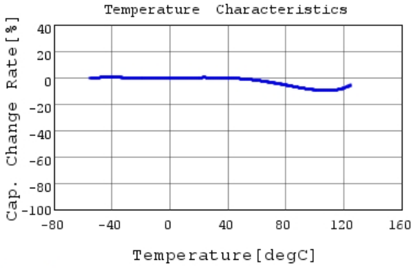
RDER72A332K0P1H03B C-Temp. capchange, DC0.0V
