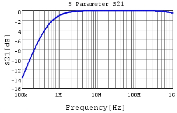
RDER72A332K0P1H03B S21 DC0V, 25degC
