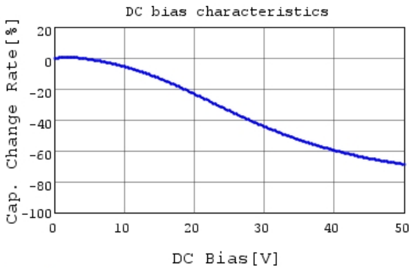
RDER71H474K1K1H03B C-DC bias capchange, 25.0
