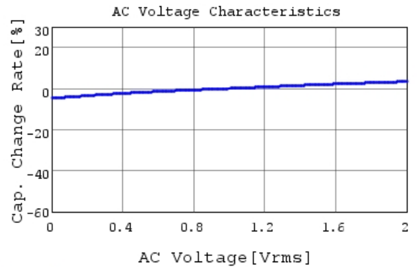
RDER71H474K1K1H03B C-AC Voltage capchange, I
