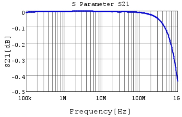
RDER71H474K1K1H03B S21 DC0V, 25degC
