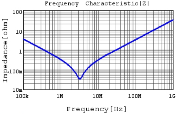
RDER71H474K1K1H03B |Z| DCOV, 25degC
