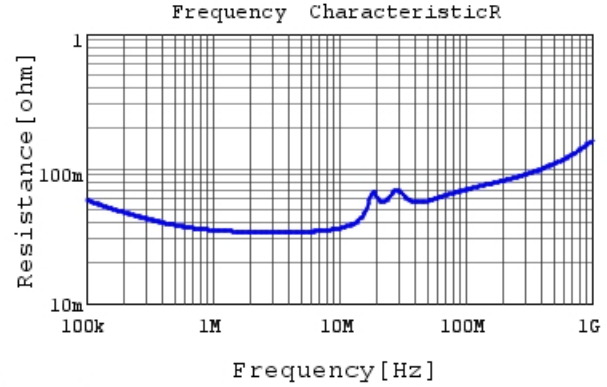
RDER71H474K1K1H03B R DCOV, 25degC
