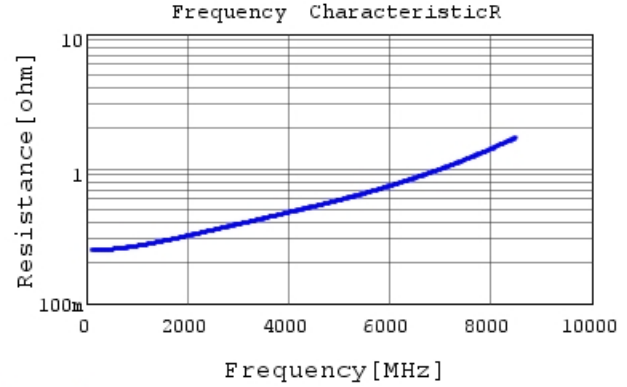
GRM0335C1H3R3CA01 R DCOV, 25degC
