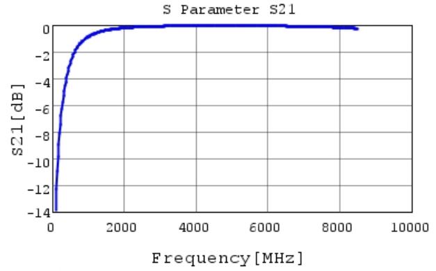
GRM0335C1H3R3CA01 S21 DCOV, 25degC
