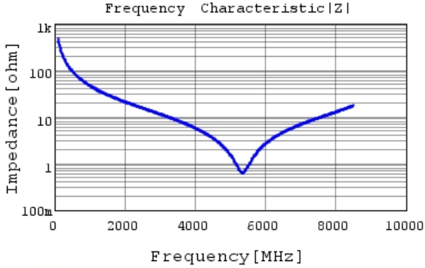
GRM0335C1H3R3CA01 |Z| DCOV, 25degC
