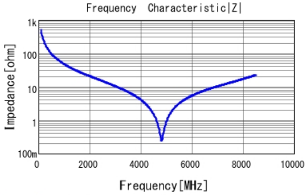
GJM1555C1H3R2BB01 |Z| DCOV, 25degC
