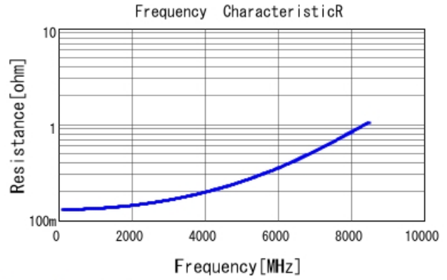
GJM1555C1H3R2BB01 R DCOV, 25degC
