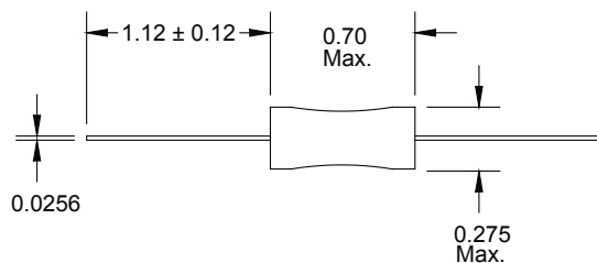
Dimensions: Inches
