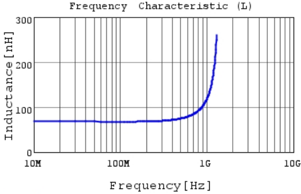
LQW2UAS68NF0C L
