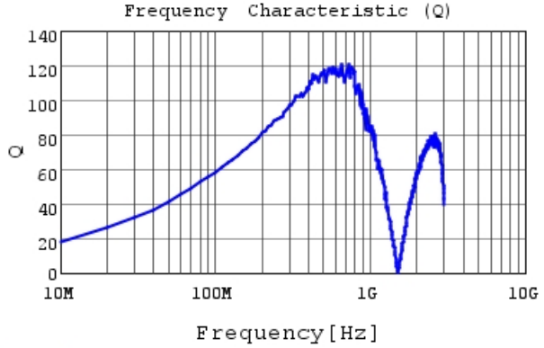
LQW2UAS68NF0C Q
