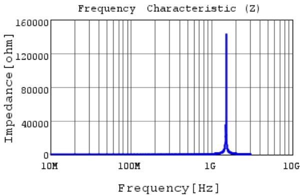
LQW2UAS68NF0C |Z|
