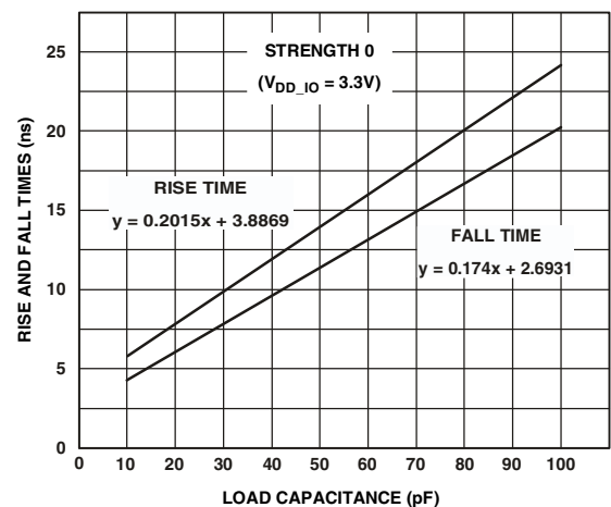
Figure 32. Typical Output Rise and Fall Time (10%-90%, V_{DD\_10} = 3.3 V) vs. Load Capacitance at Strength 0
