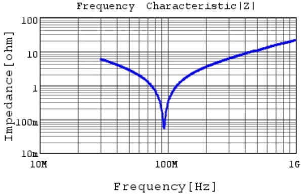
RCE5C1H821J0DBH03A |Z| DCOV, 25degC
