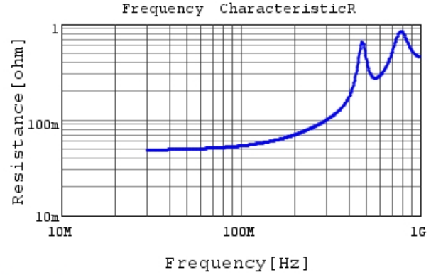
RCE5C1H821J0DBH03A R DCOV, 25degC
