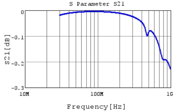
RCE5C1H821J0DBH03A S21 DCOV, 25degC
