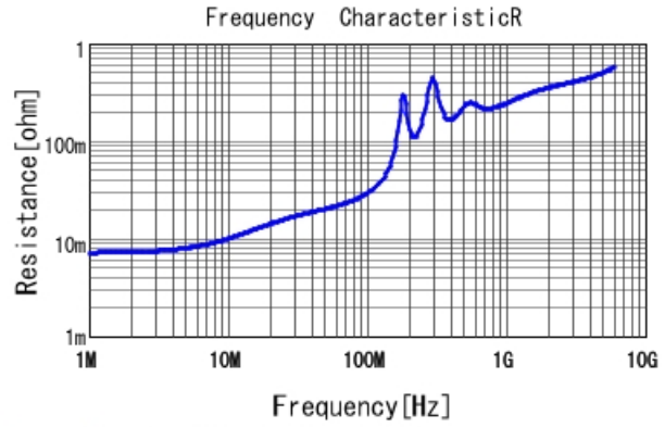
GRM2192C1H682JA01 R DCOV, 20degC
