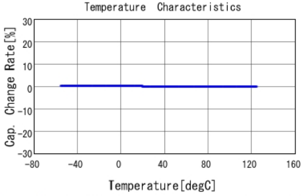
GRM2192C1H682JA01 C-Temp. capchange, DCOV, AC1Vrms
