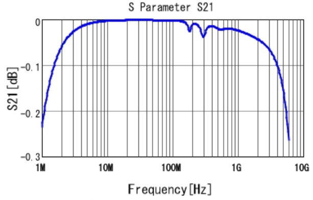
GRM2192C1H682JA01 S21 DCOV, 20degC
