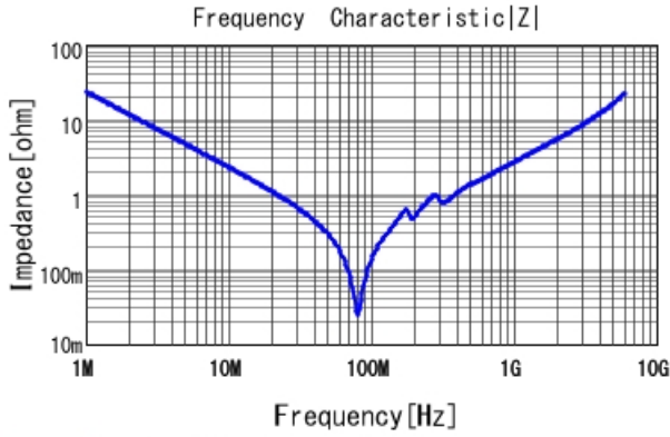
GRM2192C1H682JA01 |Z| DCOV, 20degC
