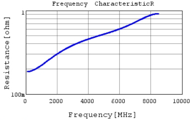
GRM0335C2A8R0DA01 R DCOV, 25degC
