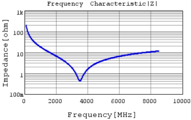
GRM0335C2A8R0DA01 |Z| DCOV, 25degC
