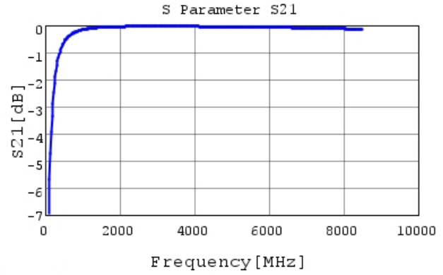
GRM0335C2A8R0DA01 S21 DCOV, 25degC
