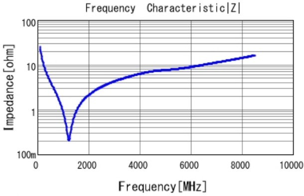
■ GRM0332C2A620JA01 |Z| DCOV, 20degC
