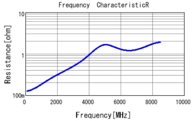
■ GRM0332C2A620JA01 R DCOV, 20degC
