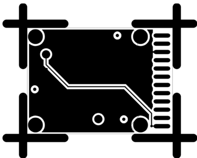
Figure 50. Layout of Circuit Side (WLCSP)
