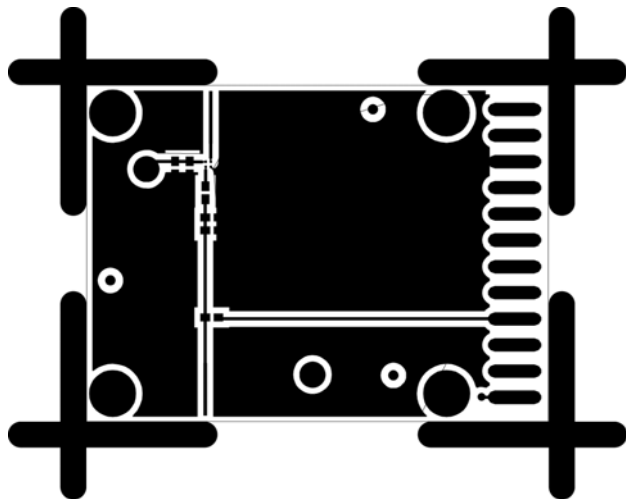
Figure 49. Layout of Component Side (WLCSP)
