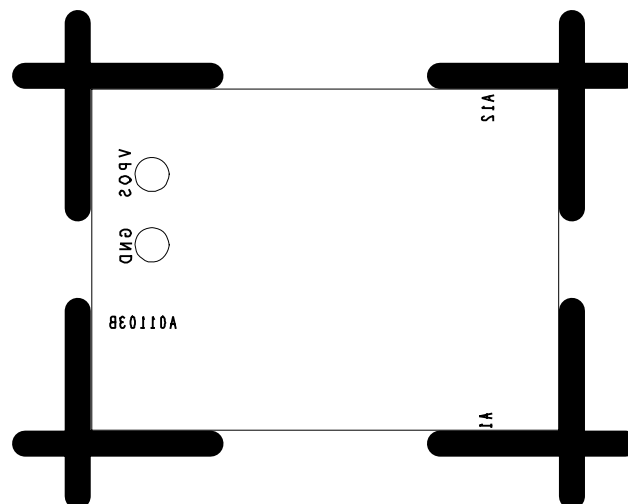
Figure 52. Silkscreen of Circuit Side (WLCSP)
