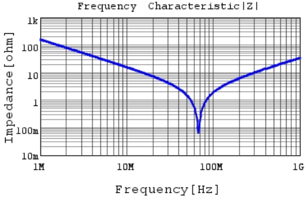
RDE5C2A102J0P1H03B |Z| DC0V, 25degC
