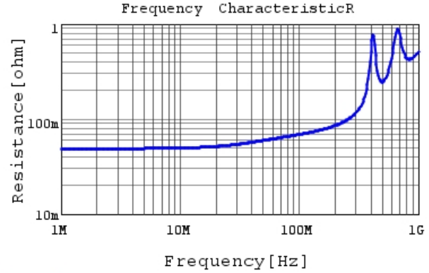
RDE5C2A102J0P1H03B R DC0V, 25degC
