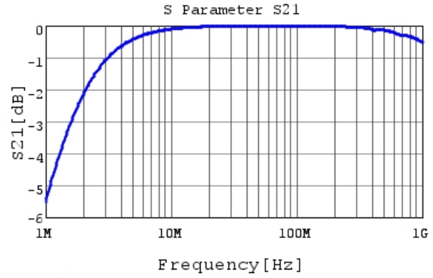
RDE5C2A102J0P1H03B S21 DCOV, 25degC
