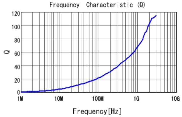
LQW15AN2N7G80 Q
