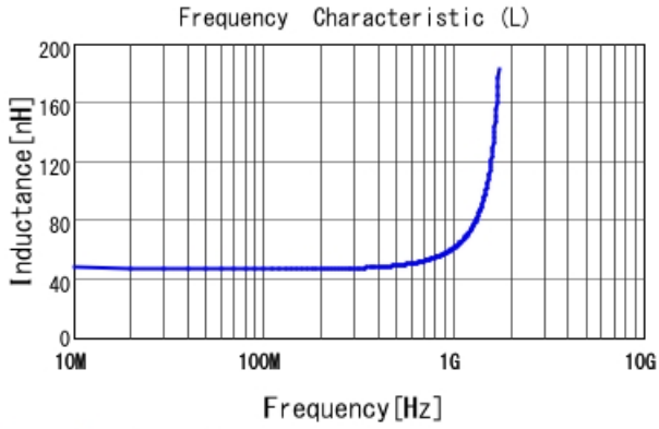
LQW2UAS47NG0C L
