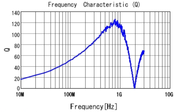
LQW2UAS47NG0C Q
