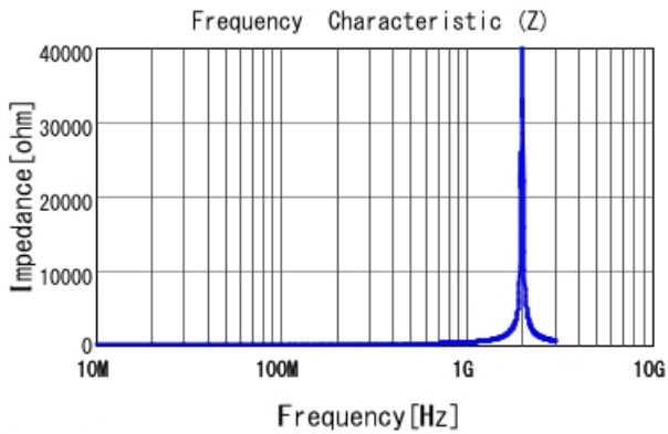
LQW2UAS47NG0C |Z|
