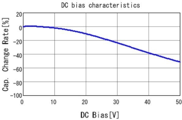
GRM188R71H683KA93 C-DC bias capchange, 25.0degC, A
