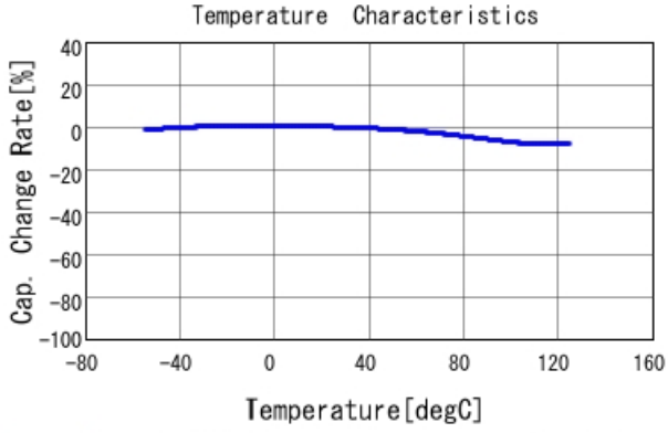
GRM188R71H683KA93 C-Temp. capchange, DC0.0V, AC1.C
