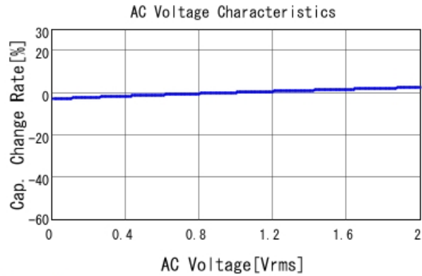
GRM188R71H683KA93 C-AC Voltage capchange, DCOV, 25
