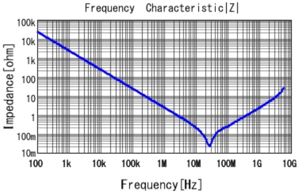
GRM188R71H683KA93 |Z| DCOV, 25degC
