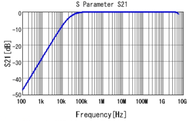
GRM188R71H683KA93 S21 DC0V, 25degC
