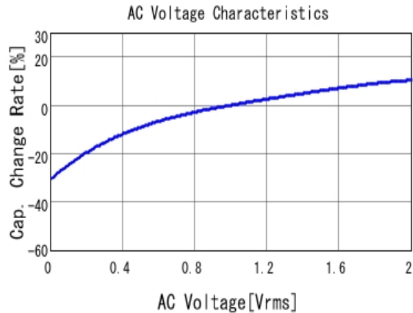
■ GRM316B31C225KA87 C-AC Voltage capchange, DCOV, 20.0d
