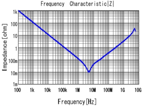
■ GRM316B31C225KA87 |Z| DCOV, 20degC
