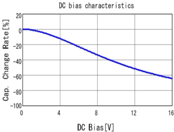
■ GRM316B31C225KA87 C-DC bias capchange, 20.0degC, AC1.
