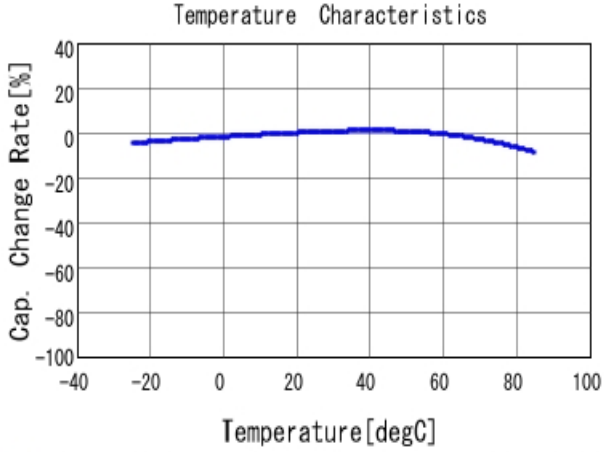
■ GRM316B31C225KA87 C-Temp. capchange, DC0.0V, AC1.0V r m
