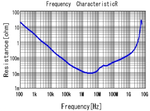
■ GRM316B31C225KA87 R DCOV, 20degC
