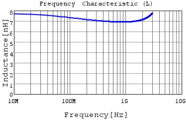
LQP02HQ6N8J02 L
