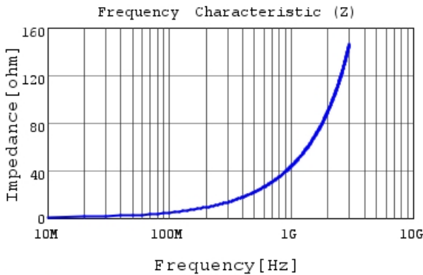
LQP02HQ6N8J02 |Z|
