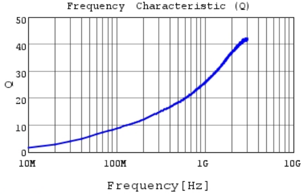
LQP02HQ6N8J02 Q
