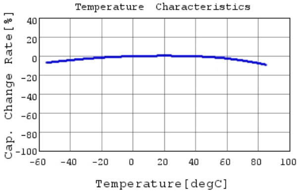
GRM033R61A223ME84 C-Temp. capchange, DC0.0V,
