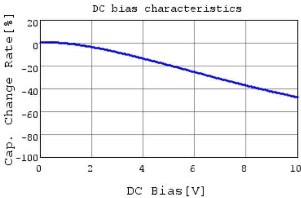
GRM033R61A223ME84 C-DC bias capchange, 25.0c
