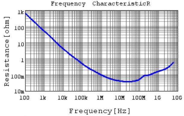
GRM033R61A223ME84 R DCOV, 25degC
