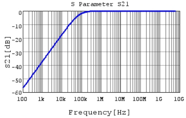
GRM033R61A223ME84 S21 DC0V, 25degC
