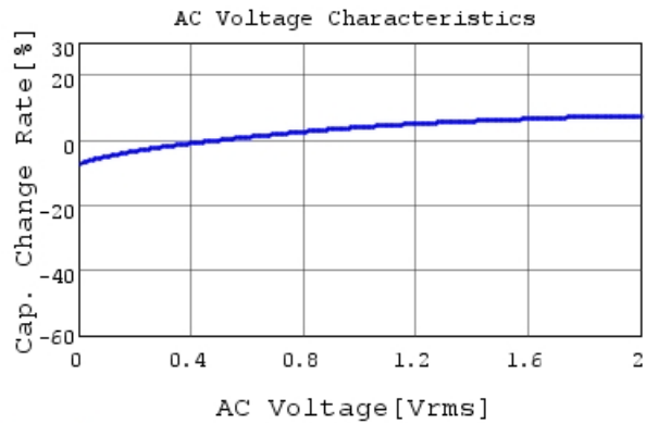
GRM033R61A223ME84 C-AC Voltage capchange, Dc
