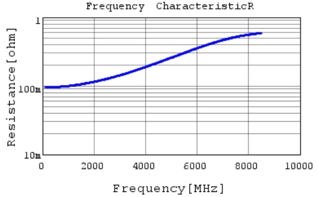
GJM0335C1E5R0CB01 R DC0V, 25degC
