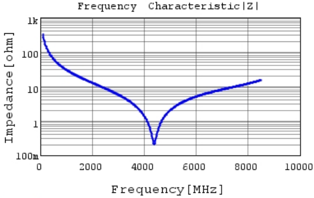
GJM0335C1E5R0CB01 |Z| DC0V, 25degC
