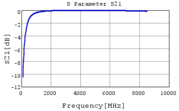
GJM0335C1E5R0CB01 S21 DCOV, 25degC
