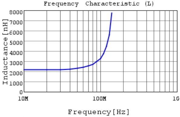
LQW2UAS2R2J0C L
