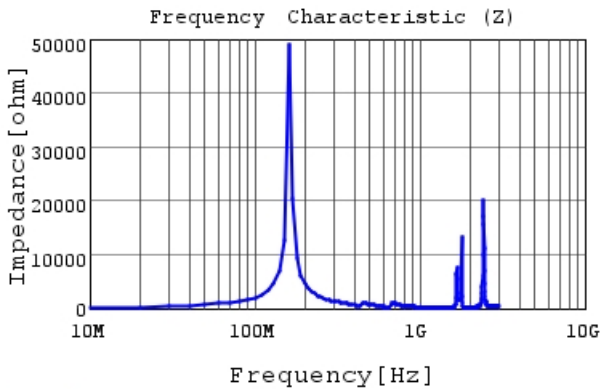
LQW2UAS2R2J0C |Z|
