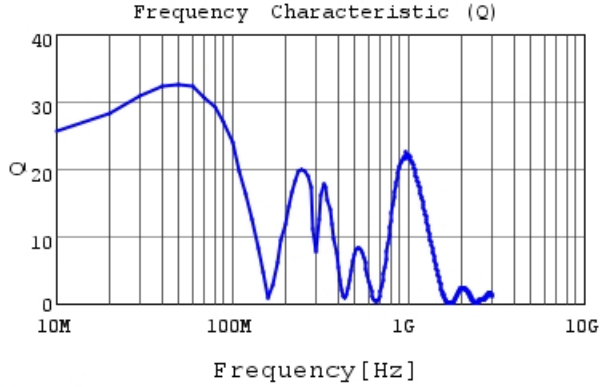
LQW2UAS2R2J0C Q
