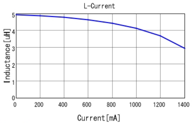
1229AS-H-4R7M L-Current 20degC
