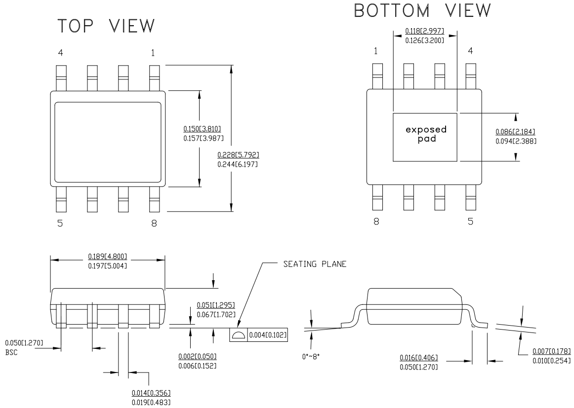
Figure 14. 8-Pin Small Outline (SOIC) Package
