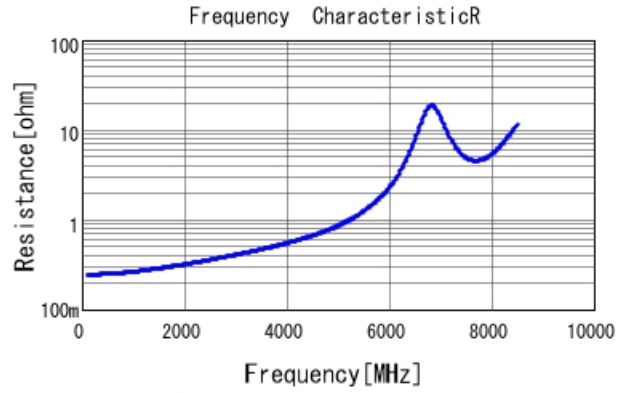
GCM1885C1H4R7CA16 R DCOV, 25degC
