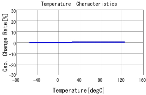
GCM1885C1H4R7CA16 C-Temp. capchange, DCOV, AC1Vrms
