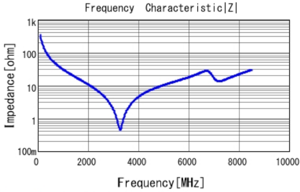
GCM1885C1H4R7CA16 |Z| DCOV, 25degC
