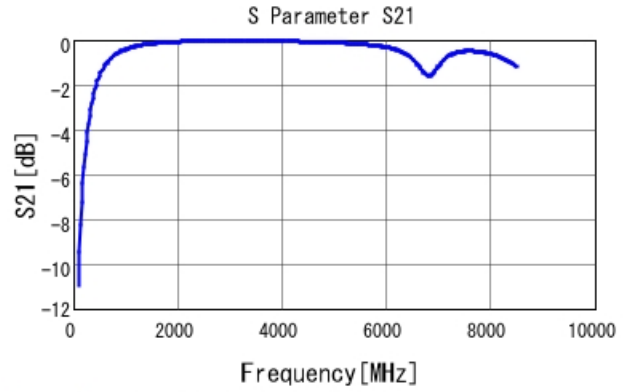
GCM1885C1H4R7CA16 S21 DCOV, 25degC
