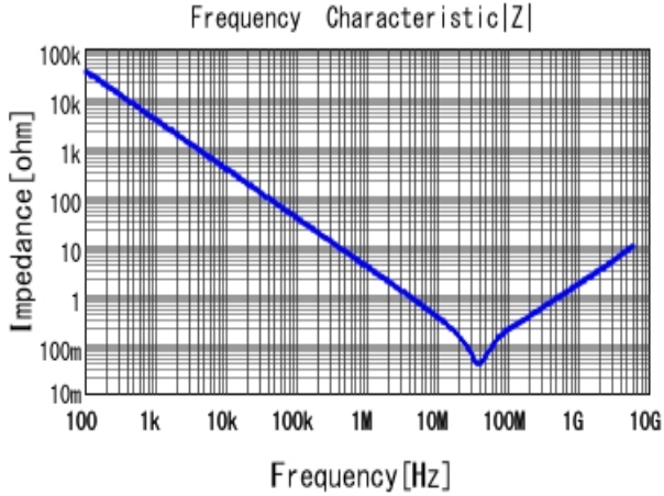
■ GRM155R71A473KA01 |Z| DCOV, 25degC
