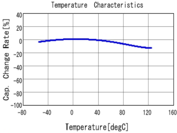
■ GRM155R71A473KA01 C-Temp. capchange, DCO. 0V, AC1.0V rm
