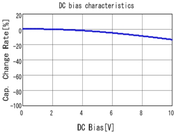
■ GRM155R71A473KA01 C-DC bias capchange, 25.0degC, AC1.
