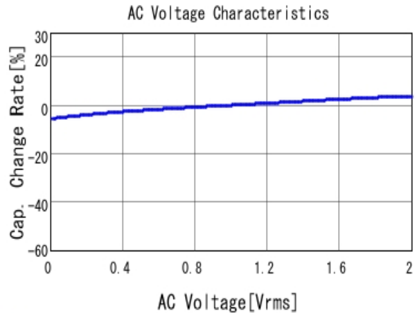
■ GRM155R71A473KA01 C-AC Voltage capchange, DCOV, 25.0d
