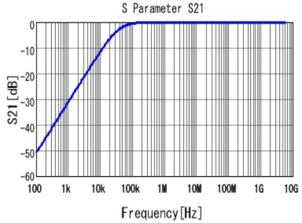
■ GRM155R71A473KA01 S21 DCOV, 25degC
