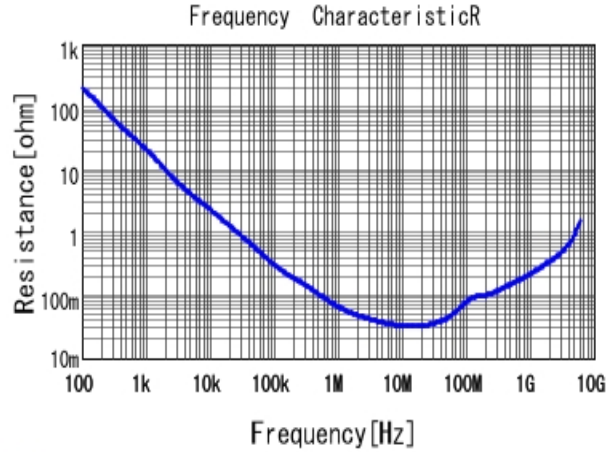
■ GRM155R71A473KA01 R DCOV, 25degC
