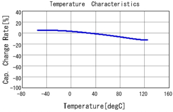
■ GRM033R71A822KA01 C-Temp. capchange, DCO. 0V, AC1. 0Vrm
