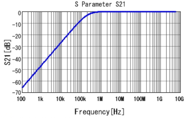
■ GRM033R71A822KA01 S21 DCOV, 25degC
