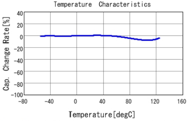
GRM188R71H471JA01 C-Temp. capchange, DC0.0V, AC1.C
