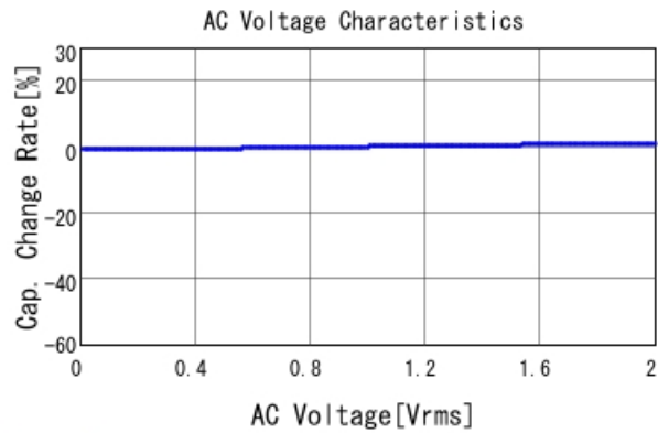
GRM188R71H471JA01 C-AC Voltage capchange, DCOV, 25
