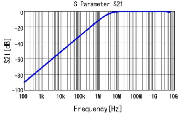
GRM188R71H471JA01 S21 DC0V, 25degC
