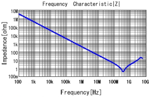
GRM188R71H471JA01 |Z| DCOV, 25degC
