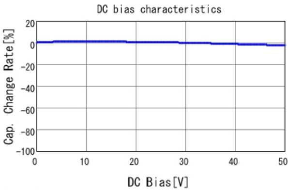
GRM188R71H471JA01 C-DC bias capchange, 25.0degC, A
