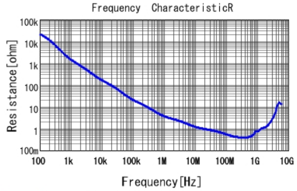
GRM188R71H471JA01 R DCOV, 25degC
