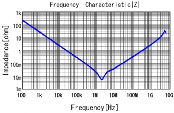
GRM319B31A106KE18 |Z| DCOV, 20degC
