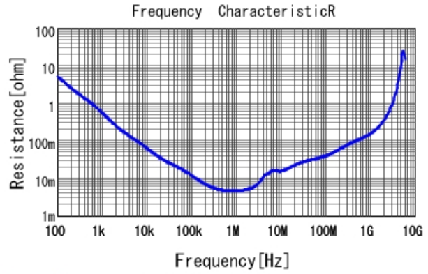
GRM319B31A106KE18 R DCOV, 20degC
