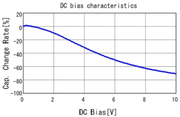
GRM319B31A106KE18 C-DC bias capchange, 20.0degC, A
