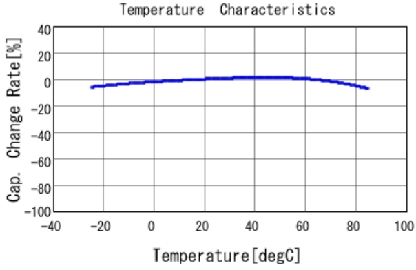
GRM319B31A106KE18 C-Temp. capchange, DC0.0V, AC0.5
