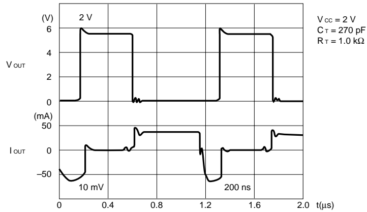
Output pin voltage and current waveforms (reference data)
