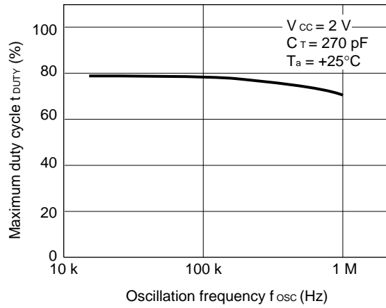
Maximum duty cycle vs. Oscillation frequency
