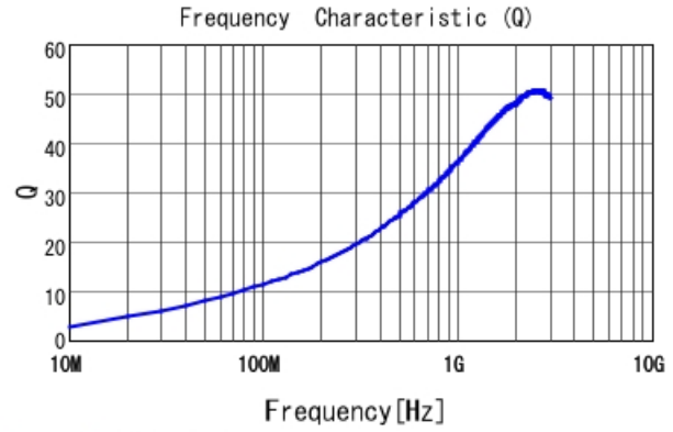
LQG15HN4N7B02 Q
