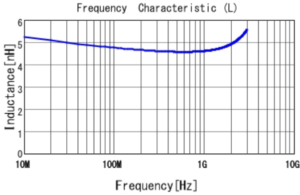
LQG15HN4N7B02 L
