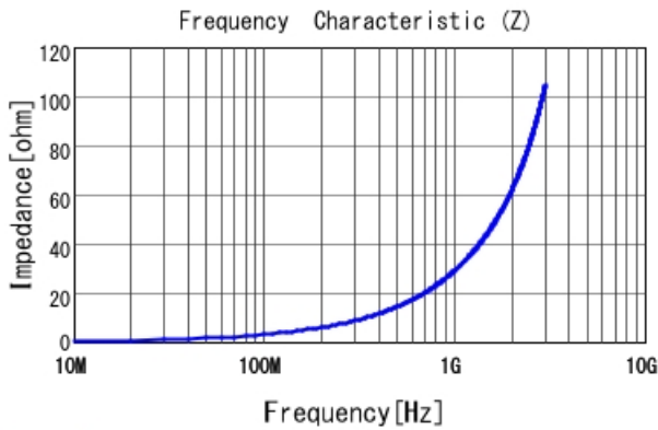
LQG15HN4N7B02 |Z|
