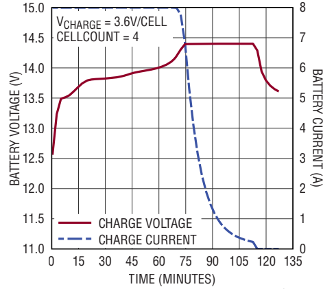
LiFePO 4 Charging Profile Voltage, Current vs Time
