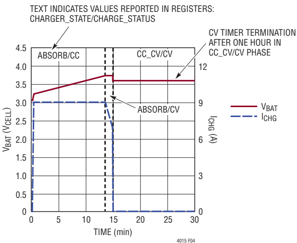
Figure 4. LiFePO 4 Fast Charge Charging Profile
