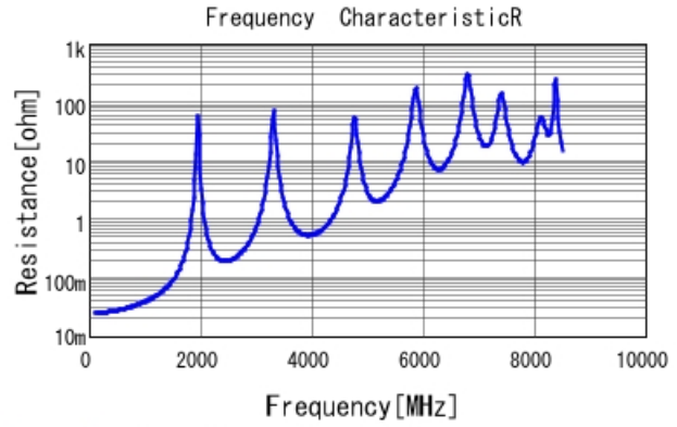
GQM22M5C2H680JB01 R DCOV, 25degC
