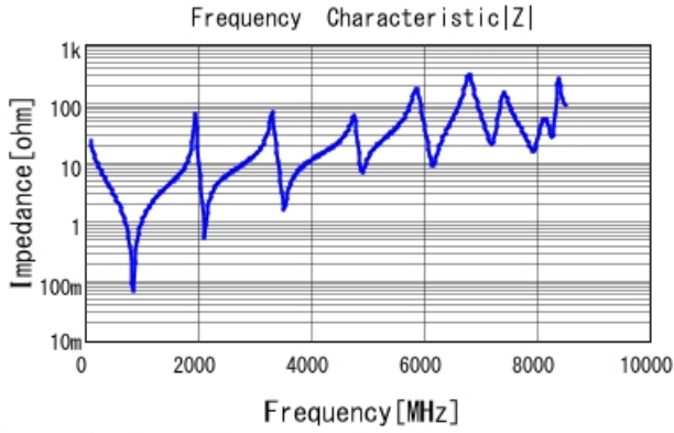
GQM22M5C2H680JB01 |Z| DCOV, 25degC
