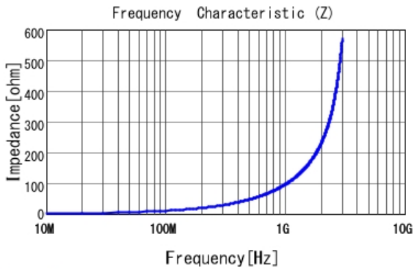
LQP02TN15NJ02 |Z|
