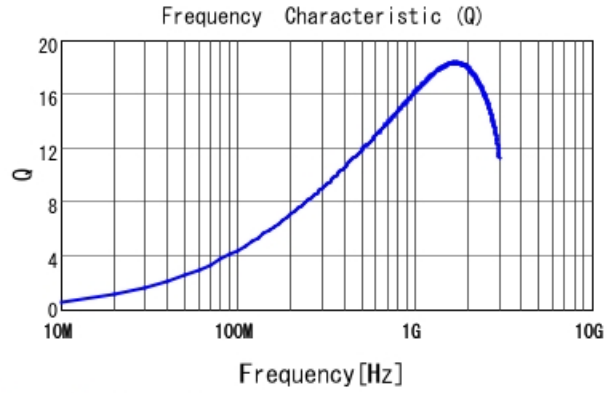
LQP02TN15NJ02 Q
