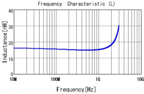
LQP02TN15NJ02 L
