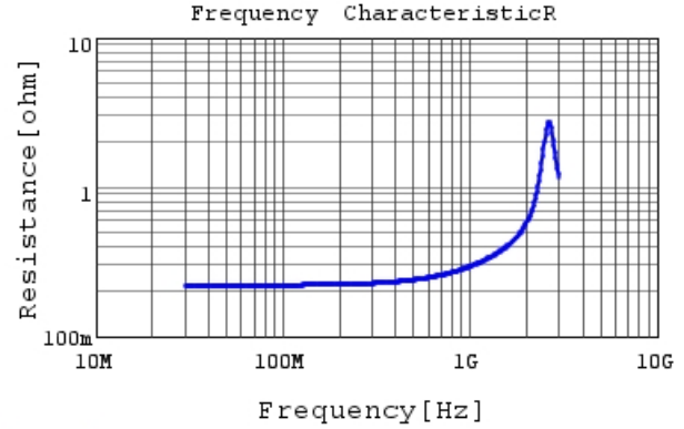
RDE5C2A330J0M1H03A R DC0V, 25degC
