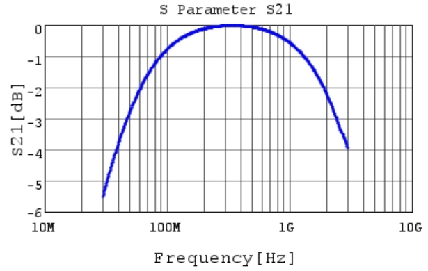
RDE5C2A330J0M1H03A S21 DCOV, 25degC
