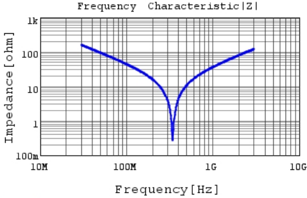
RDE5C2A330J0M1H03A |Z| DC0V, 25degC
