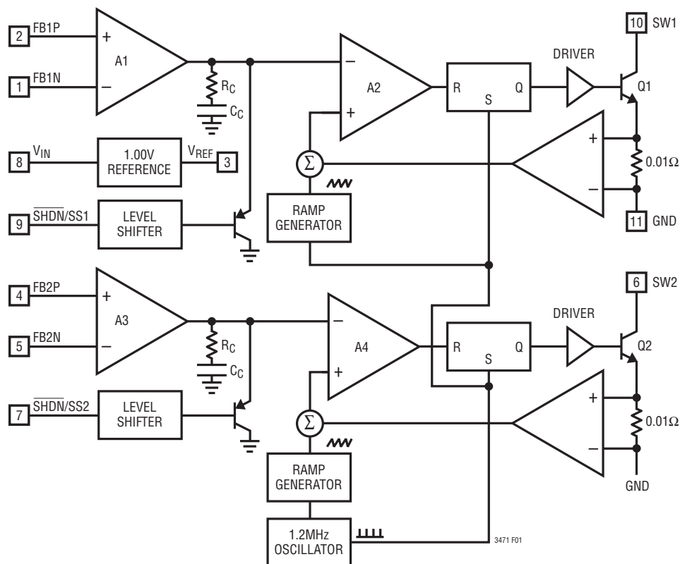
Figure 1. Block Diagram
