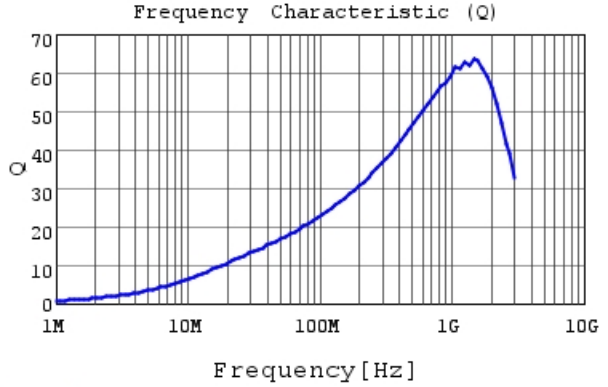
LQW15AN39NJ8Z Q
