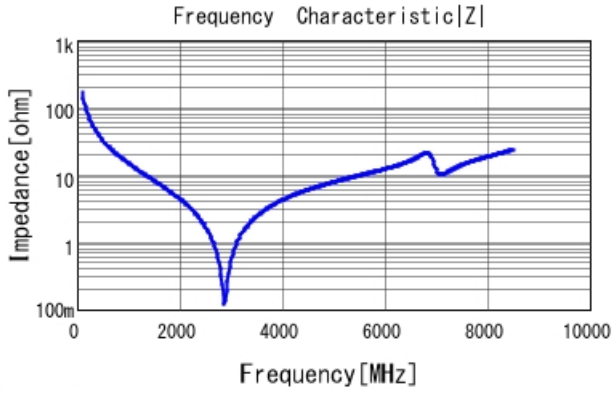
GJM1555C1H9R5WB01 |Z| DCOV, 25degC
