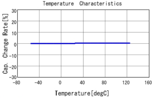
GJM1555C1H9R5WB01 C-Temp. capchange, DC0V, AC1Vrms
