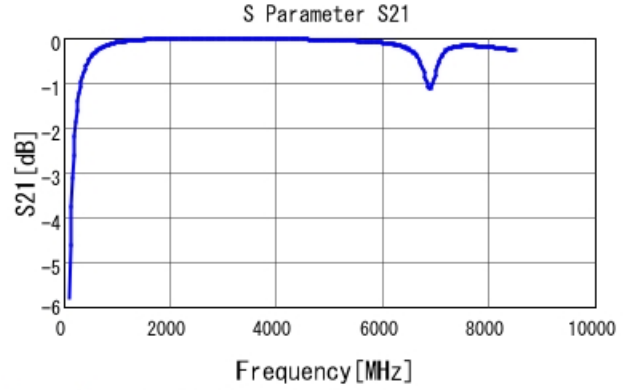
GJM1555C1H9R5WB01 S21 DC0V, 25degC
