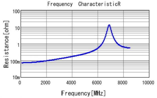
GJM1555C1H9R5WB01 R DCOV, 25degC
