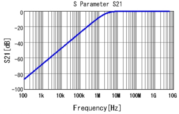
■ GRM033B31H681KA12 S21 DCOV, 20degC
