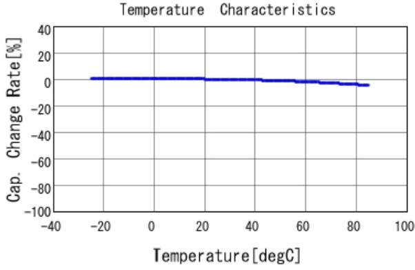
■ GRM033B31H681KA12 C-Temp. capchange, DCO. 0V, AC1. 0Vrm
